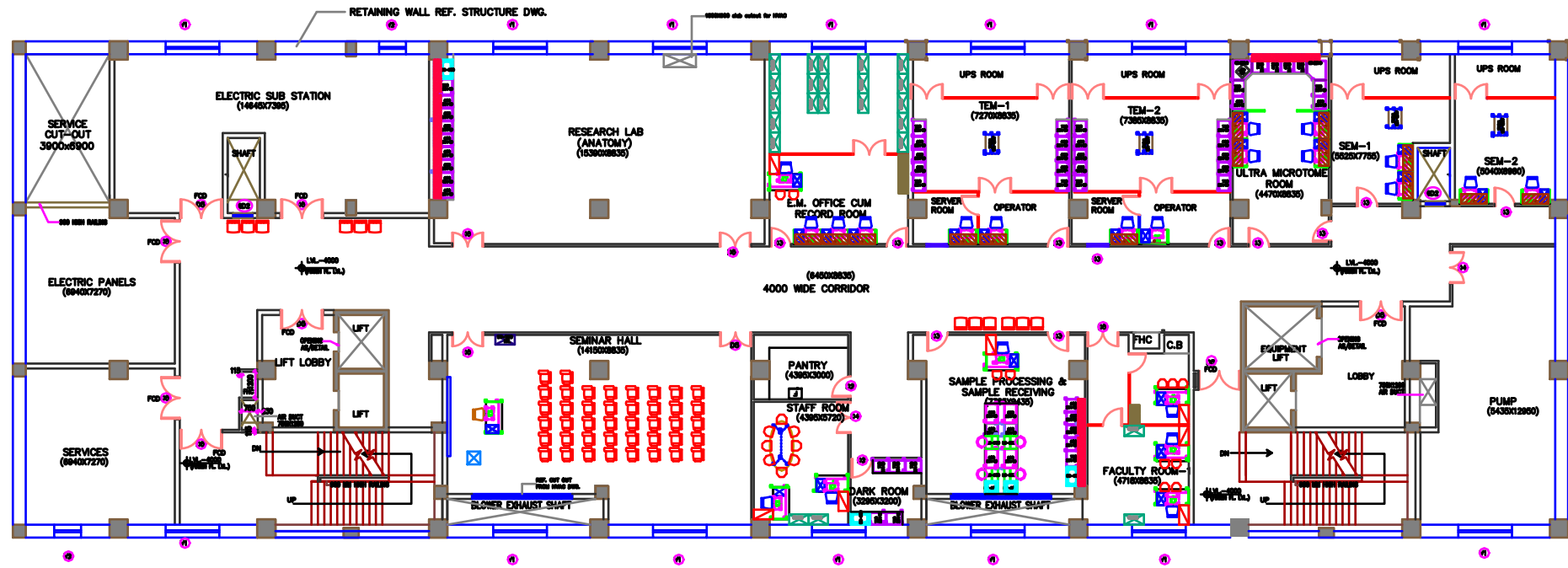
BASEMENT-1 FLOOR PLAN (ANATOMY/EM FACILITY)
