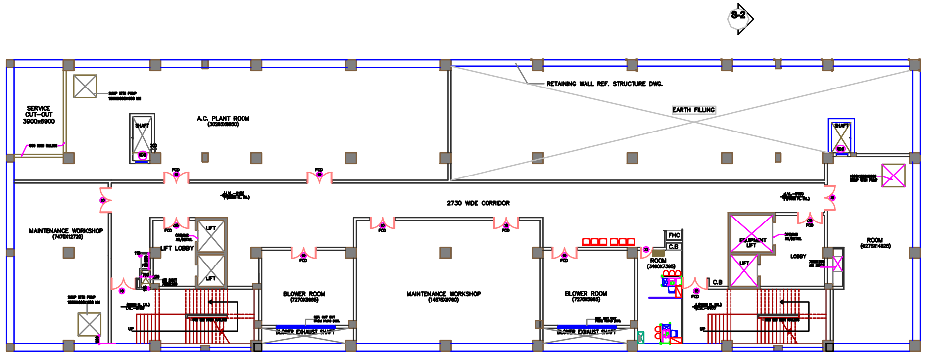
BASEMENT-2 FLOOR PLAN (SERVICES)
